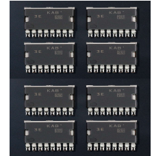
MOS-FET switch On-resistance: 0.84mΩ
